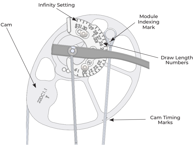
Figure 1 - Diamond Edge XT draw length adjustment
