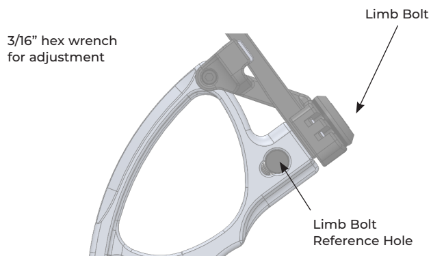
Figure 2. Draw Weight Adjustment
